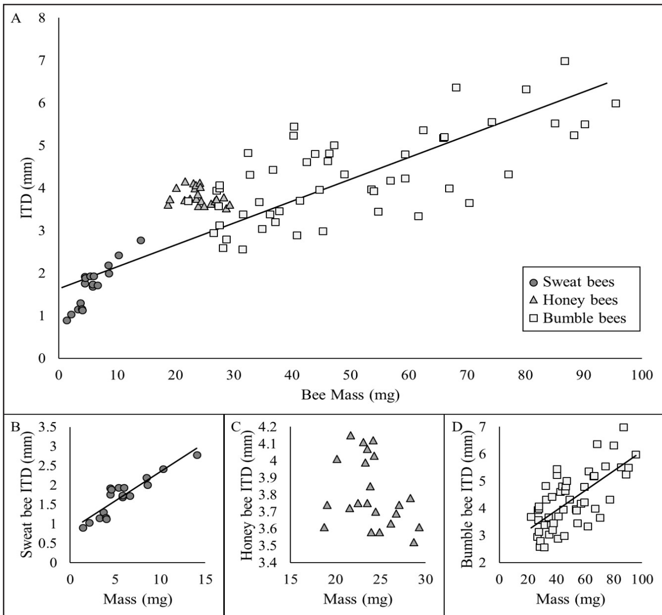
FIGURE 1. Relationship between intertegular distance (ITD) and dry mass across and within species. (A) ITD was significantly associated with dry mass for all individuals sampled ( p < 0.001 , R^2 = 0.77 ). (B) Sweat bee ITD was significantly associated with dry mass ( p < 0.001 , R^2 = 0.93 ). (C) Honey bee ITD was not associated with dry mass ( p = 0.17 , R^2 = 0.39 ). (D) Bumble bee ITD was significantly associated with dry mass ( p < 0.001 , R^2 = 0.54 ). This figure reports conditional R^2 values.
